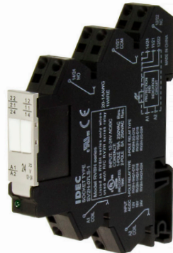
Spring Clamp Terminal
