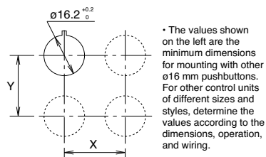
ø40 mm Mushroom
