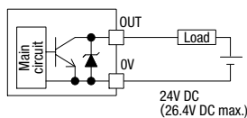
External output (OUT0 to 3)
