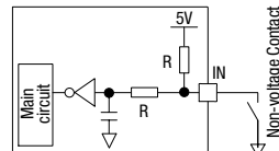
External input (IN0, 1)
