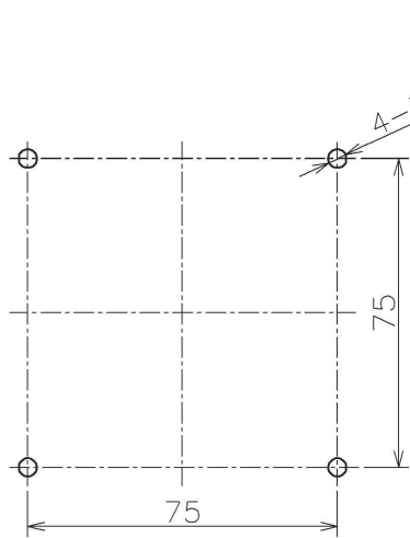
Mounting hole machining drawing
